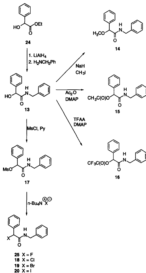
Scheme 1. Preparation of substituted N -benzyl 2-phenylacetamides.
