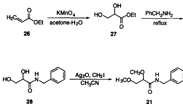
Scheme 2. Preparation of compounds 21 and 28 .
